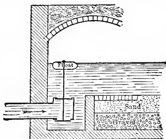
FIG. 10.—REGULATION OF INFLOW USED AT MÜGSEL, BERLIN.
